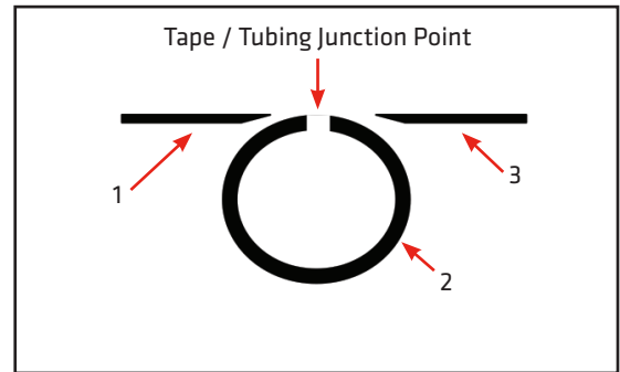
Figure 2: Duct Configuration over cable coil
